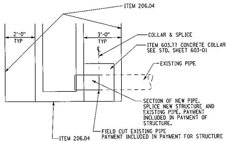
DETAIL FOR PLACING A NEW STRUCTURE OVER AN EXISTING PIPE NOT TO SCALE
