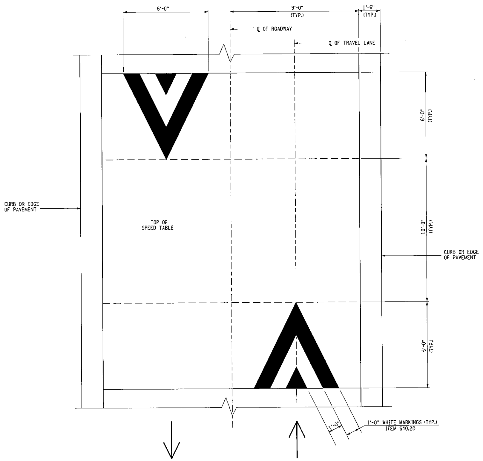
TYPICAL PAVEMENT MARKINGS SCALE: 1/4" = 1'-0"
