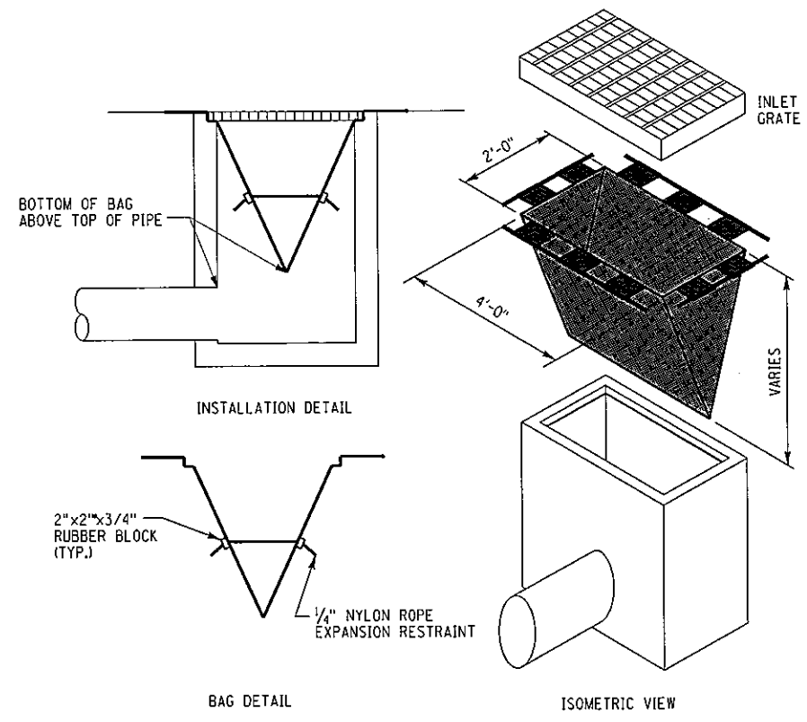
TEMPORARY SEDIMENT FILTER BAG DETAIL ITEM 209.11...10 NOT TO SCALE
