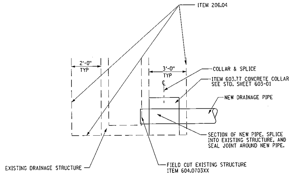
DETAIL FOR PLACING A NEW DRAIN PIPE INTO AN EXISTING STRUCTURE NOT TO SCALE
