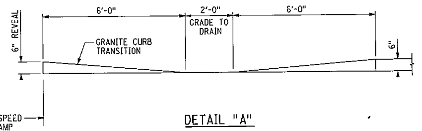
DETAIL "A" CURB TRANSITION TO DRAINAGE OUTLET NOT TO SCALE
