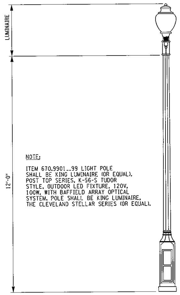
LIGHT POLE DETAIL ITEM 670.9901...99 NOT TO SCALE
